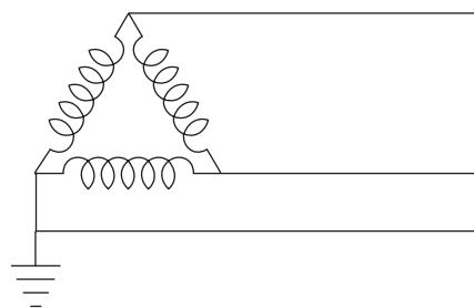
Figure 1: System Diagram, 3 \phi W Ground B \phi Delta
