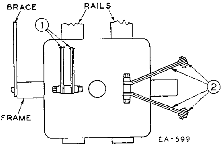
Fig. 16. Detail similar to Fig. 15 but with steel frame directly in way of intertier connector (2). Note connector bent away from frame. Also wrap connector with insulating tape where contact might be possible. Applies to 2 tier rack only.
