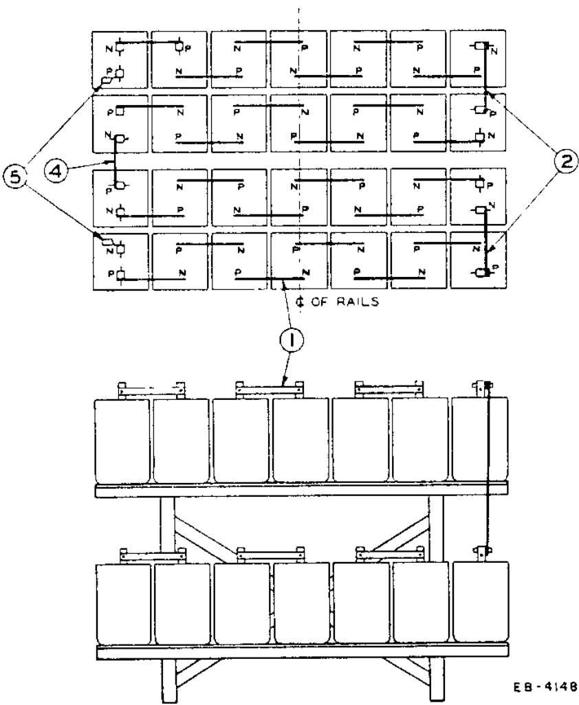
Fig. 11 Two racks back to back, with odd number of cells in place. Upper view shows intercell connection (1) and side view interstep connectors (2), and interrack connector (4). (For even number of cells, see Fig. 9 for connector arrangement.)
