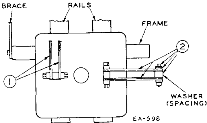
Fig. 15. Detail showing intertier connector (2) when four pieces of connector are used. (Connector could be made of one, two or three pieces also.) (Note clearance between frame and connector. See Fig. 16 for unfavorable location of frame. Applies to 2 tier racks only.)
