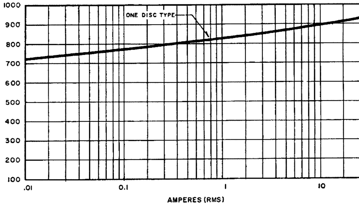
Figure 4: Typical Volt-ampere characteristic of Varistor in Type KAB Relay (RMS).
