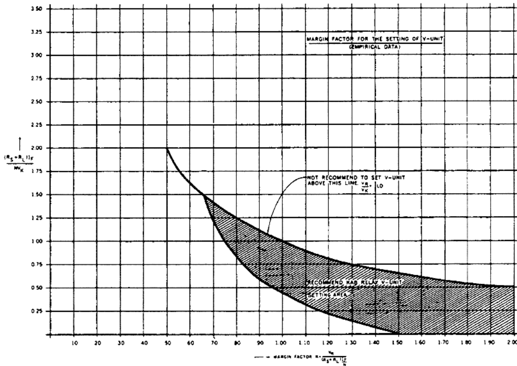
Figure 5: Margin Factor for V-Unit Setting
