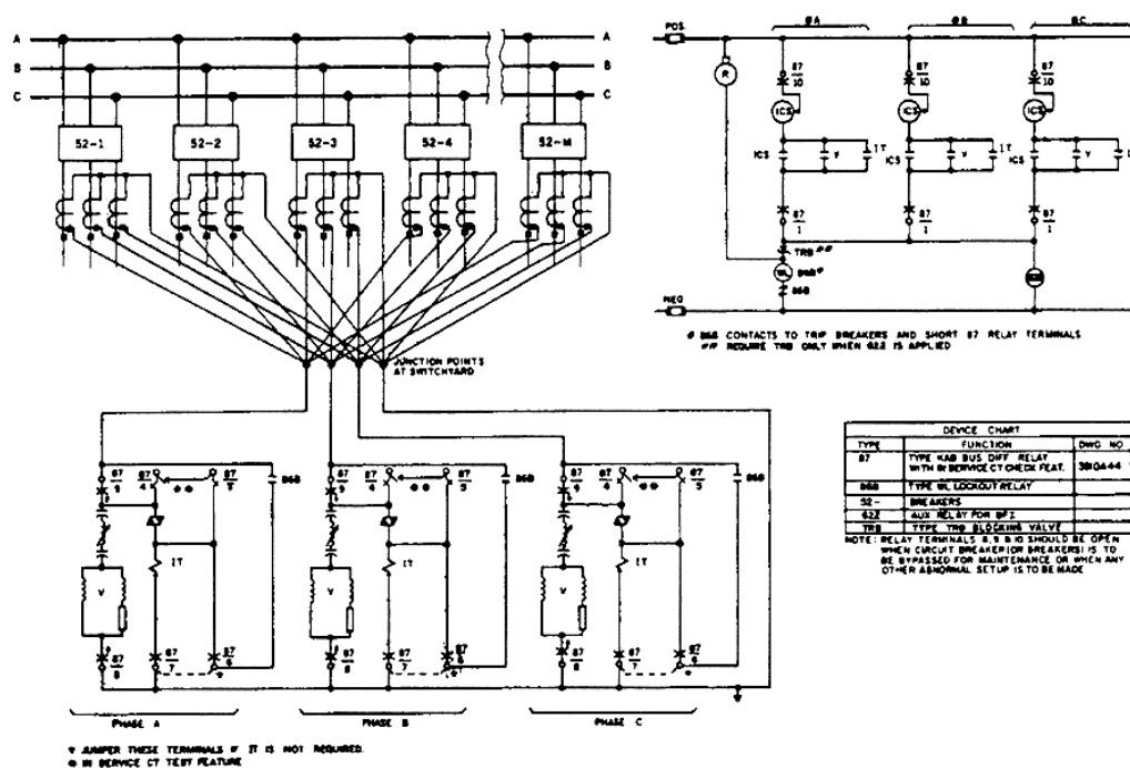
Figure 7: External Connections
