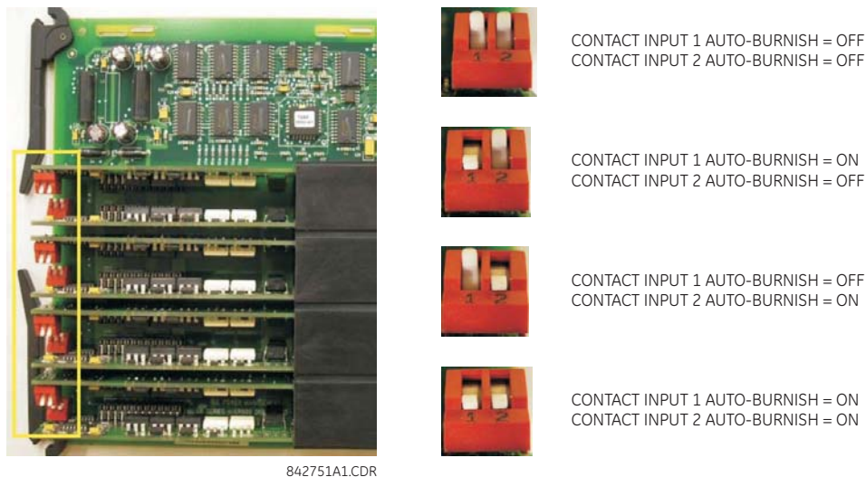
Figure 3-16: AUTO-BURNISH DIP SWITCHES
