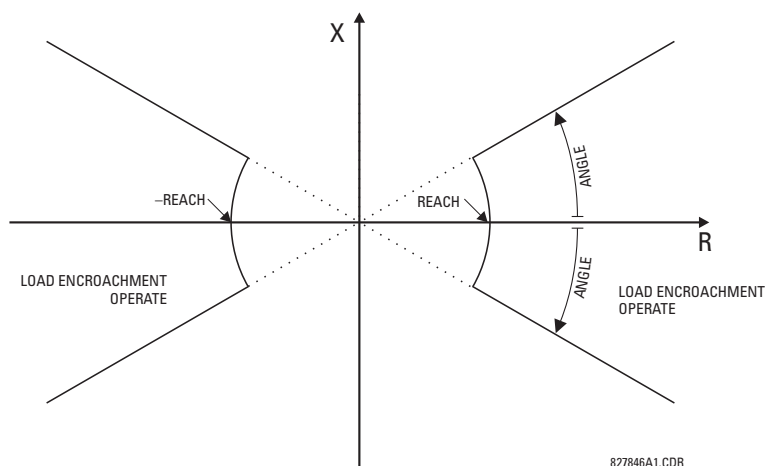
Figure 5-59: LOAD ENCROACHMENT CHARACTERISTIC
