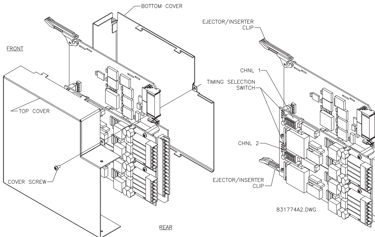
Figure 3-37: IEEE C37.94 TIMING SELECTION SWITCH SETTING
