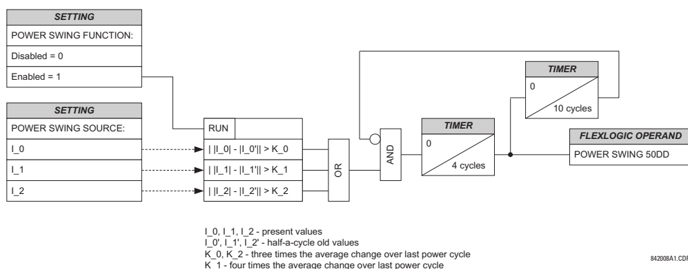
Figure 5-57: POWER SWING DETECT SCHEME LOGIC (2 of 3)
