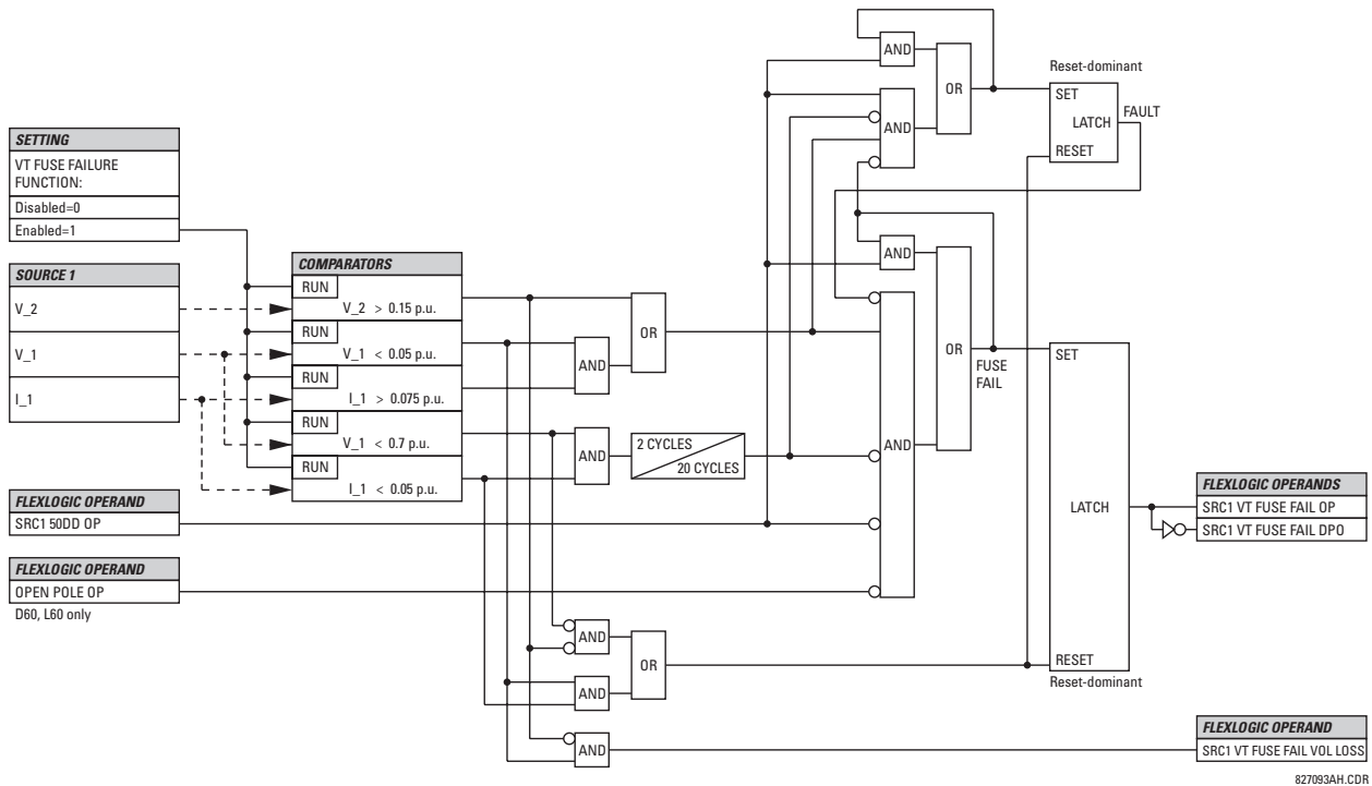
Figure 5-98: VT FUSE FAIL SCHEME LOGIC
