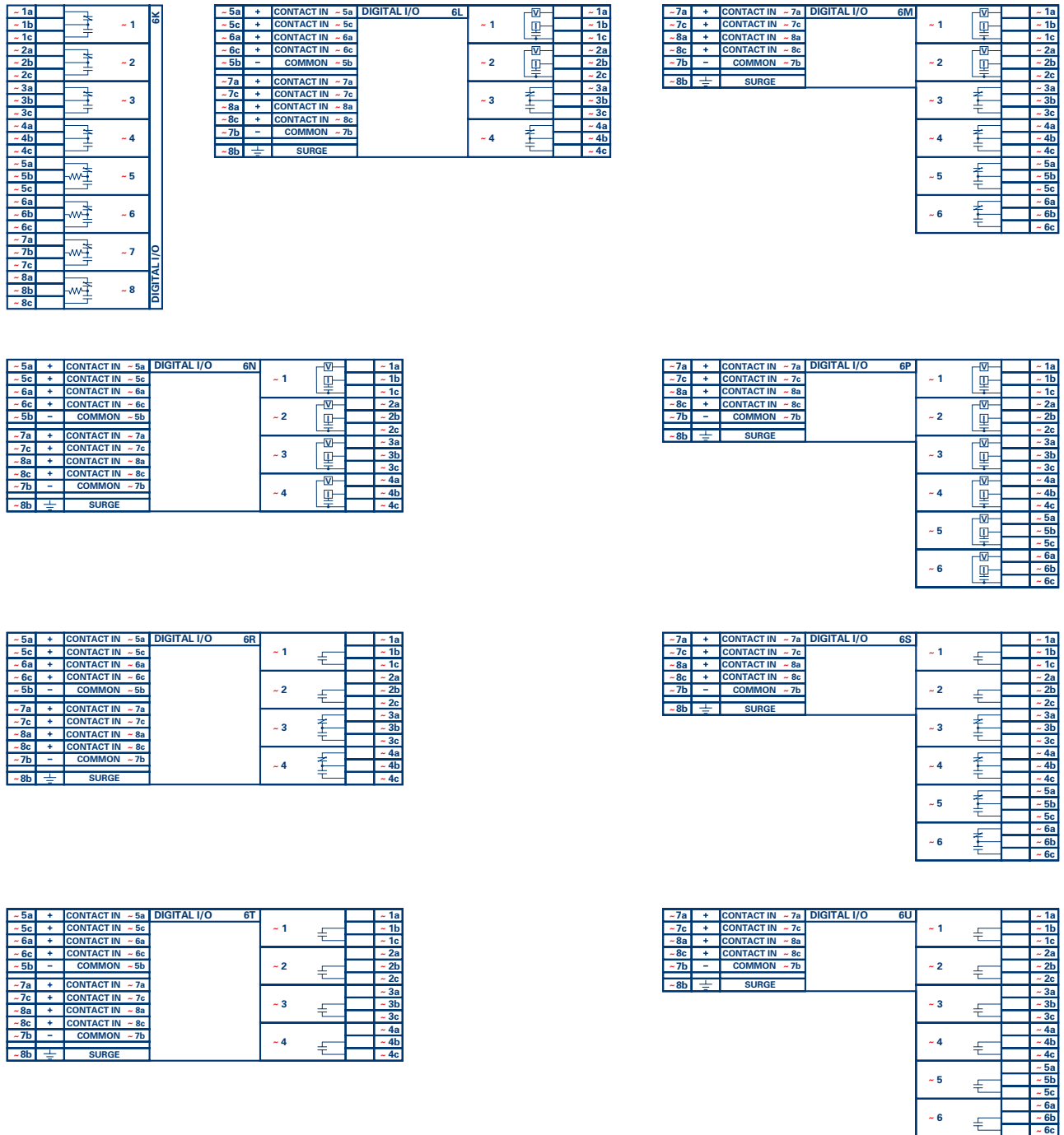
Figure 3-13: DIGITAL INPUT/OUTPUT MODULE WIRING (2 of 2)
