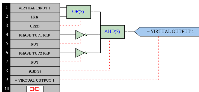
Figure 5-84: EXAMPLE FLEXLOGIC™ CONTROL OF A SETTINGS GROUP
