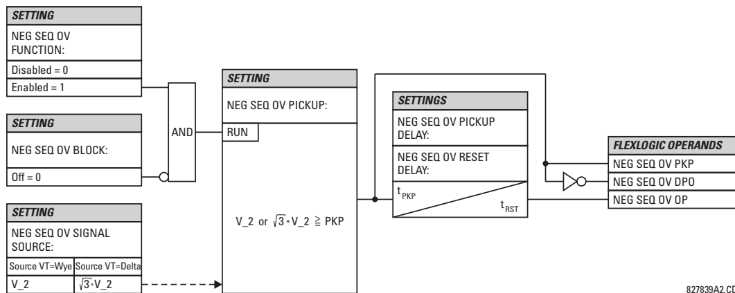
Figure 5-81: NEG SEQ OV SCHEME LOGIC
