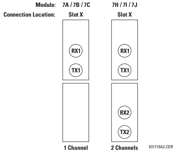
Figure 3–26: LED AND ELED FIBER MODULES
