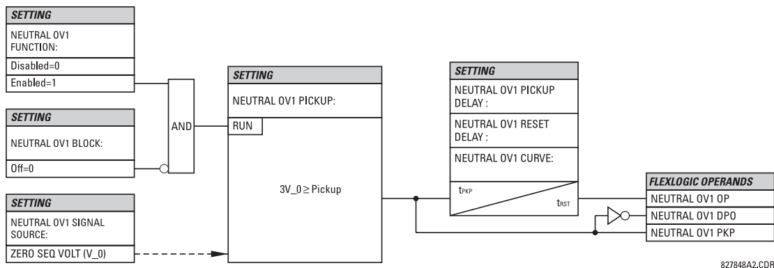
Figure 5-80: NEUTRAL OVERVOLTAGE1 SCHEME LOGIC
