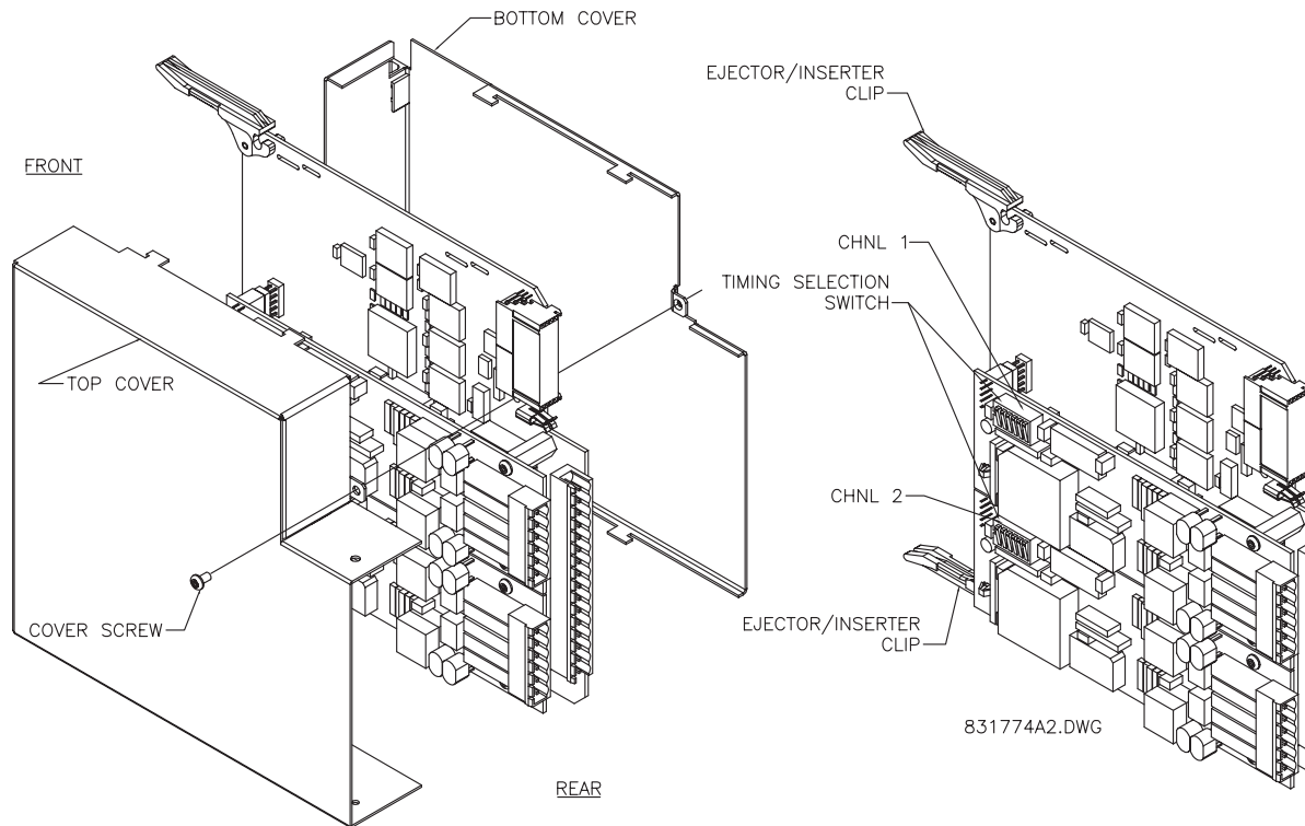
Figure 3-30: G.703 TIMING SELECTION SWITCH SETTING
