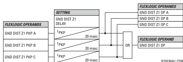
Figure 5-50: GROUND DISTANCE Z1 TO Z3 OP SCHEME
