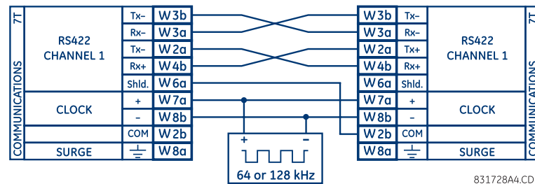
Figure 3-32: TYPICAL PIN INTERCONNECTION BETWEEN TWO RS422 INTERFACES
