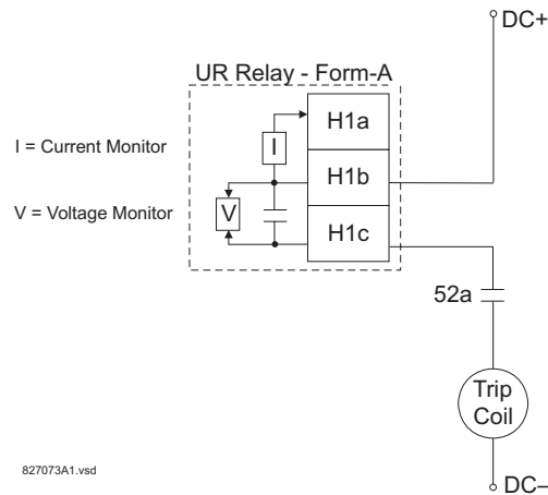
Figure 5-93: TRIP CIRCUIT EXAMPLE 1
