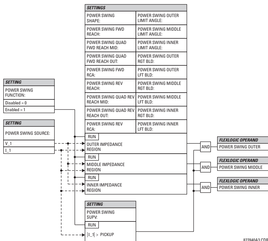
Figure 5-56: POWER SWING DETECT SCHEME LOGIC (1 of 3)
