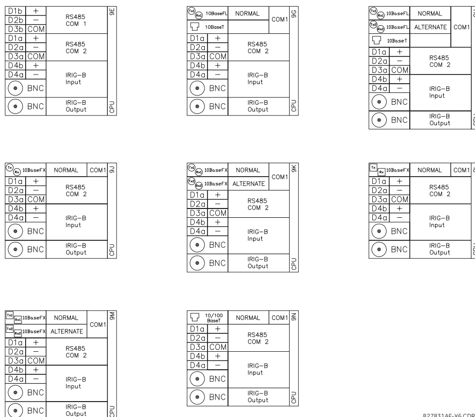
Figure 3-19: CPU MODULE COMMUNICATIONS WIRING
