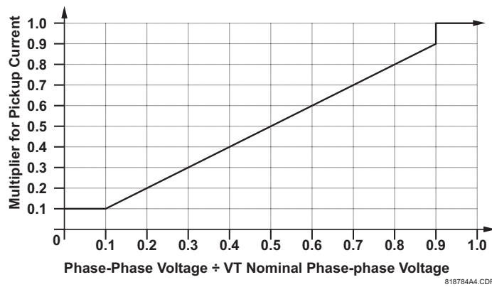
Figure 5-62: PHASE TOC VOLTAGE RESTRAINT CHARACTERISTIC
