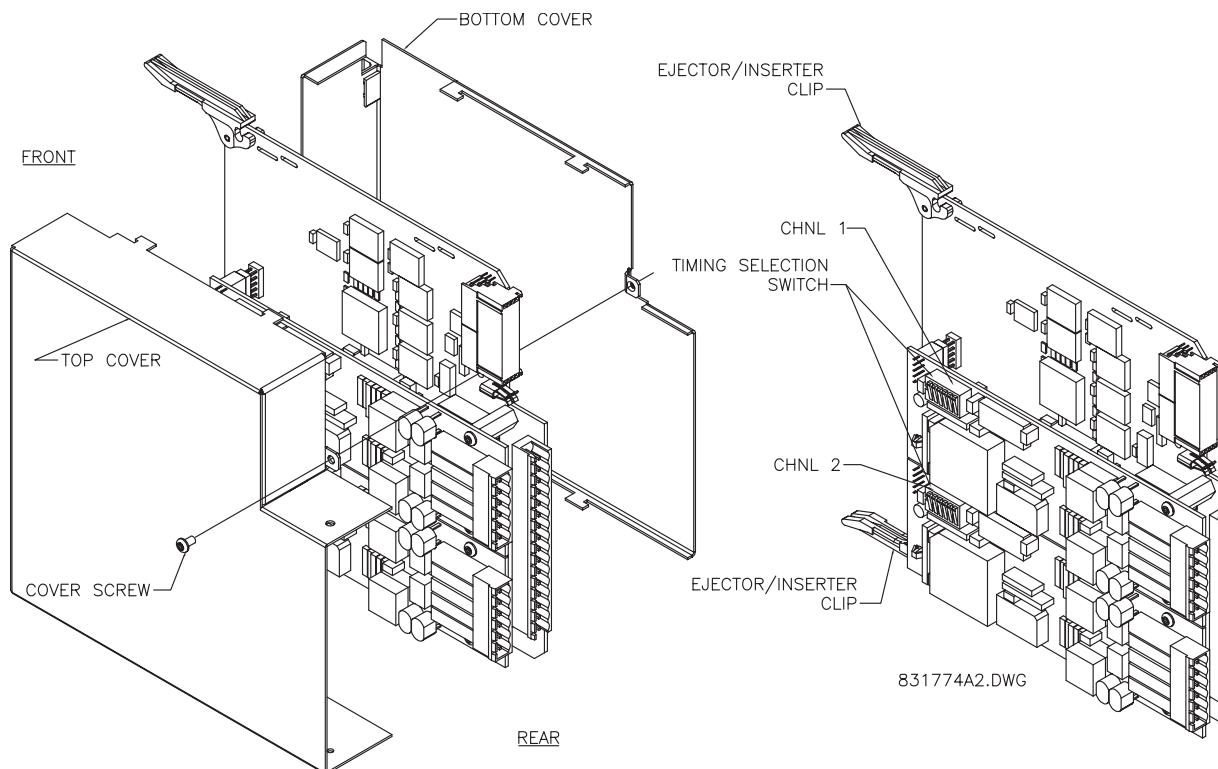
Figure 3–38: C37.94SM TIMING SELECTION SWITCH SETTING
