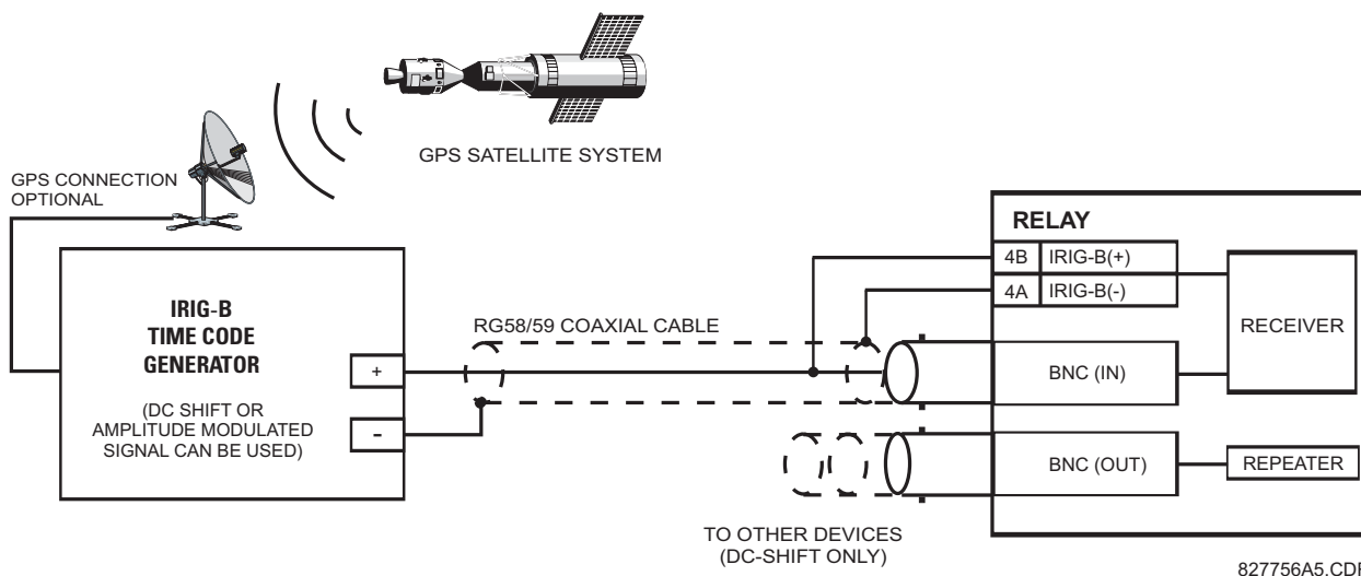
Figure 3-21: IRIG-B CONNECTION
