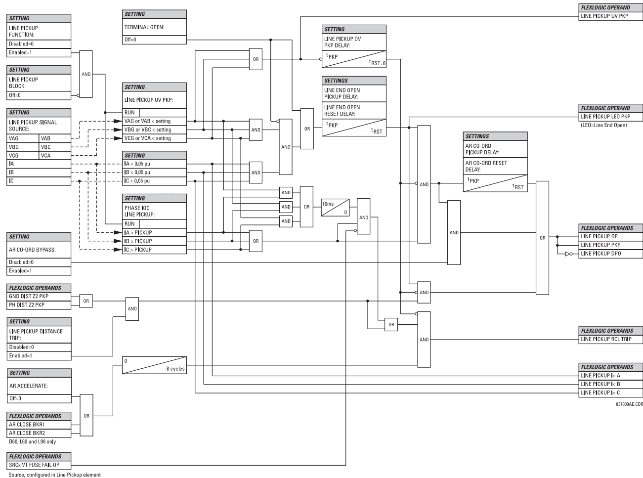
Figure 5-37: LINE PICKUP SCHEME LOGIC
