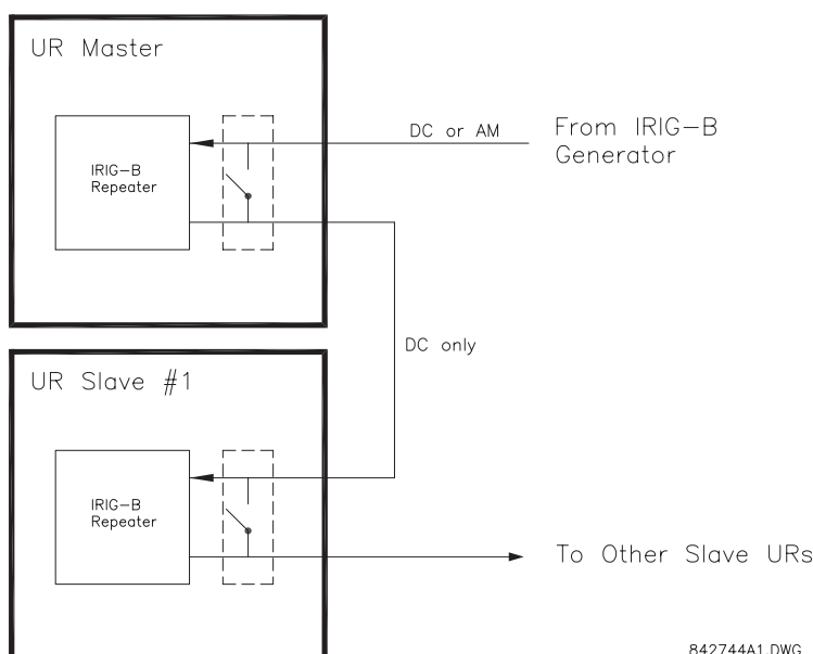
Figure 3-22: IRIG-B REPEATER
