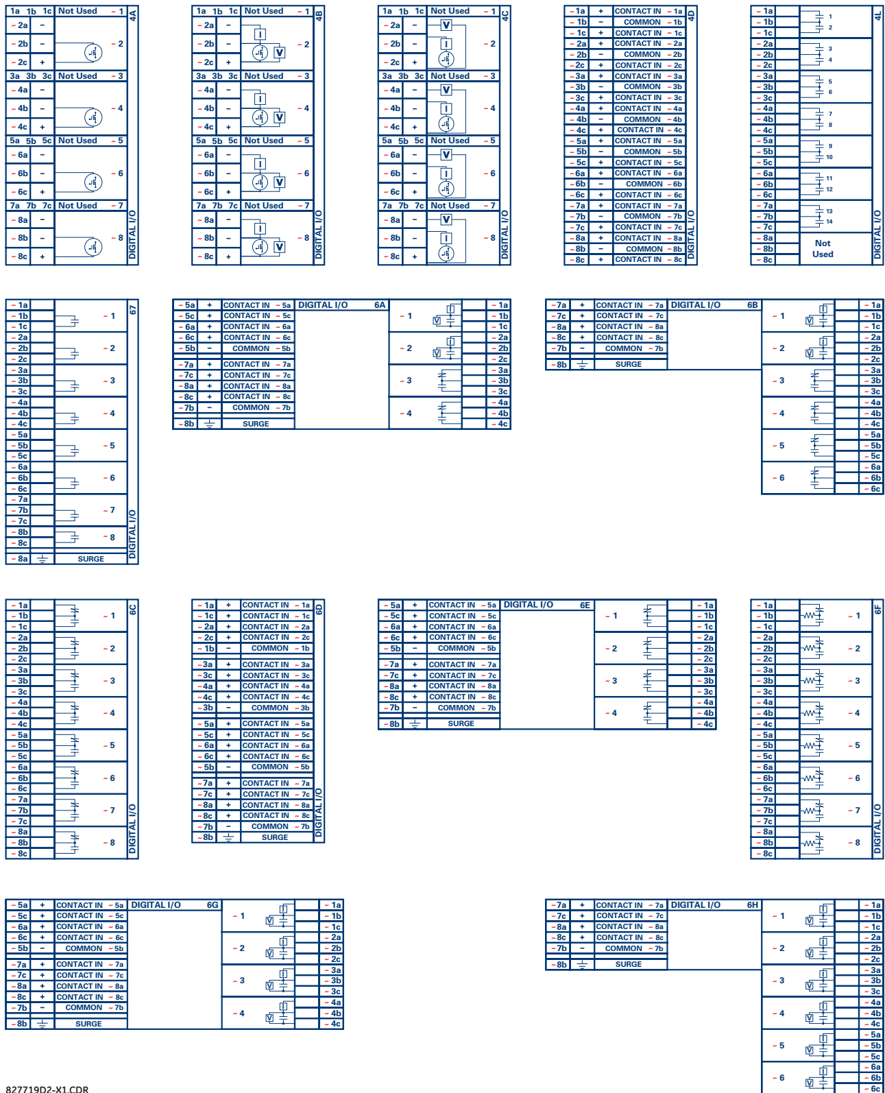
Figure 3-12: DIGITAL INPUT/OUTPUT MODULE WIRING (1 of 2)
