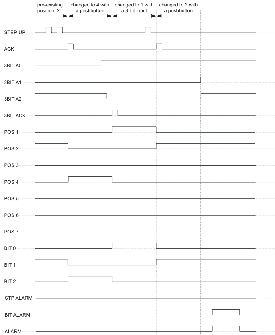
Figure 5–86: ACKNOWLEDGE MODE
