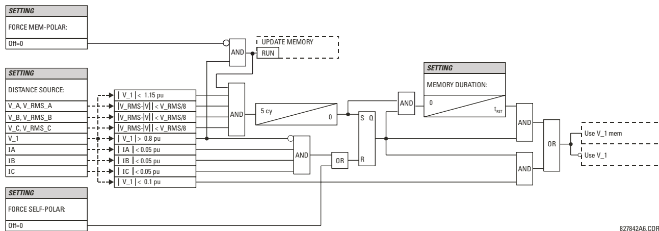
Figure 5–38: MEMORY VOLTAGE LOGIC
