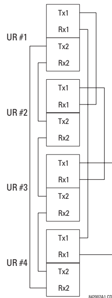
Figure 3–24: DIRECT INPUT/OUTPUT DUAL CHANNEL CONNECTION
