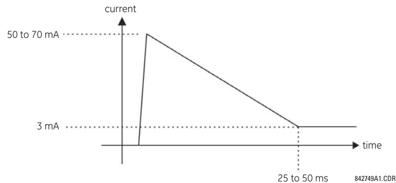
Figure 3-15: CURRENT THROUGH CONTACT INPUTS WITH AUTO-BURNISHING
