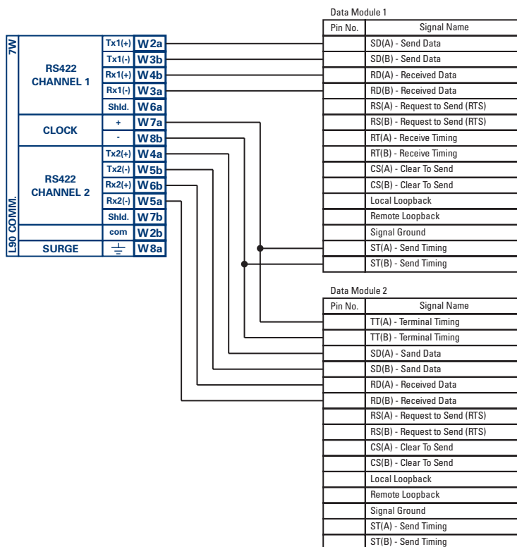
Figure 3–33: TIMING CONFIGURATION FOR RS422 TWO-CHANNEL, 3-TERMINAL APPLICATION
