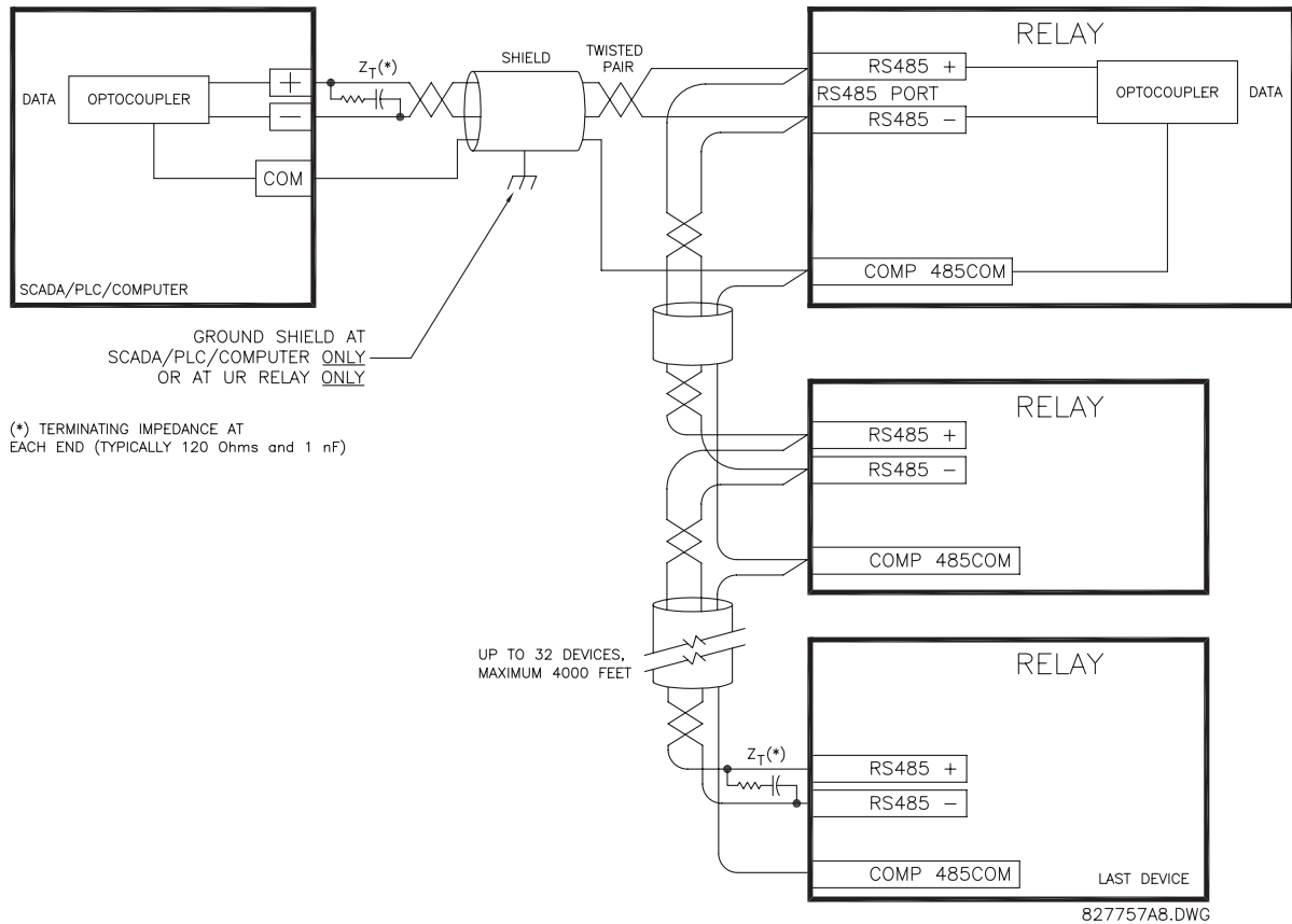
Figure 3-20: RS485 SERIAL CONNECTION
