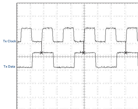
Figure 3–34: CLOCK AND DATA TRANSITIONS
