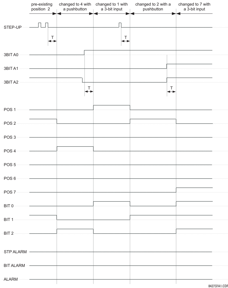
Figure 5–85: TIME-OUT MODE
