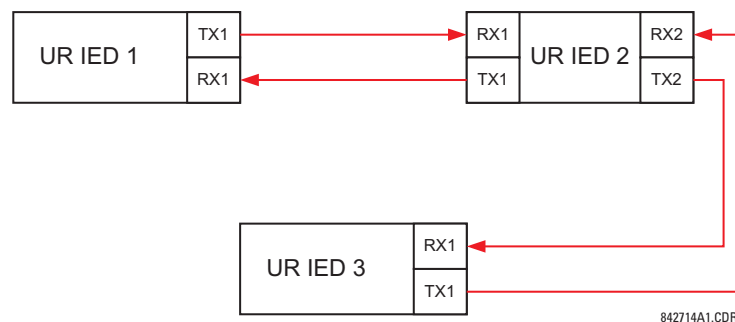
Figure 5-104: SINGLE-CHANNEL OPEN-LOOP CONFIGURATION
