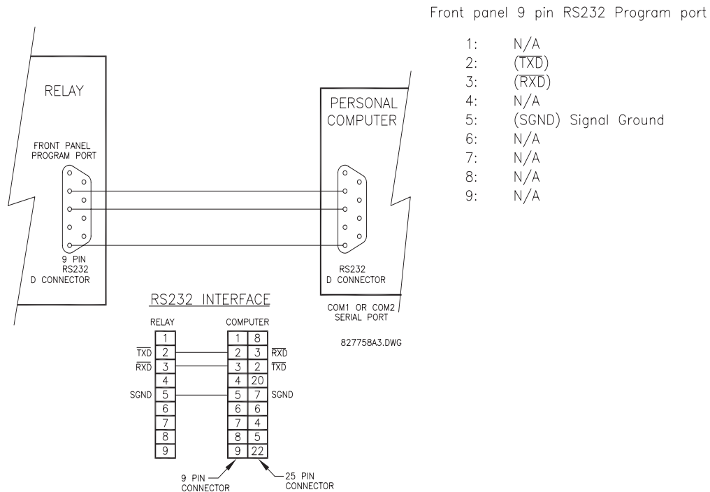
Figure 3–18: RS232 FACEPLATE PORT CONNECTION
