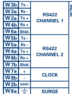
Figure 3-31: RS422 INTERFACE CONFIGURATION
