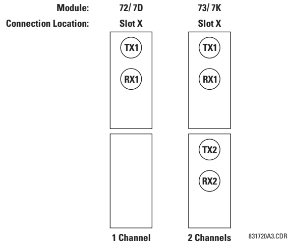
Figure 3–27: LASER FIBER MODULES
