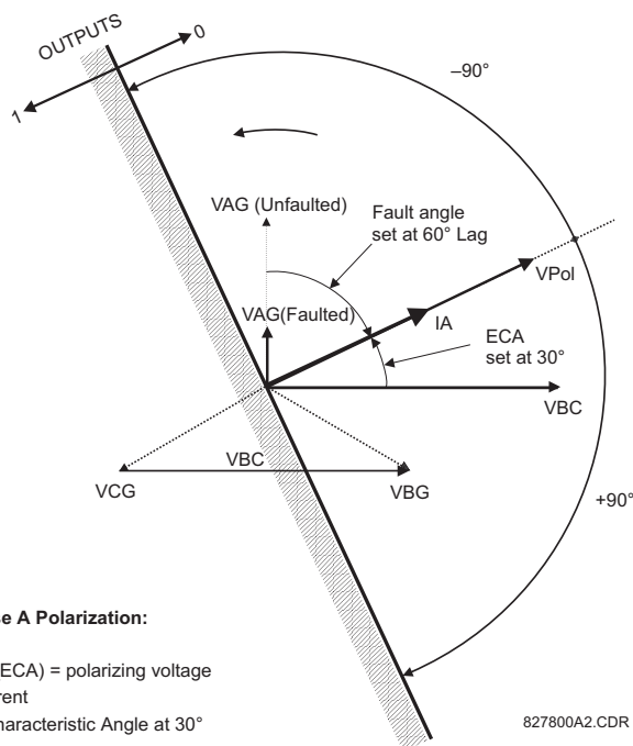
Figure 5-65: PHASE A DIRECTIONAL POLARIZATION
