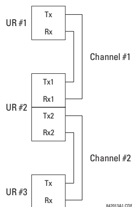
Figure 3–25: DIRECT INPUT/OUTPUT SINGLE/DUAL CHANNEL COMBINATION CONNECTION
