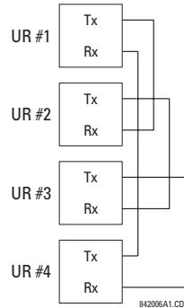
Figure 3–23: DIRECT INPUT/OUTPUT SINGLE CHANNEL CONNECTION
