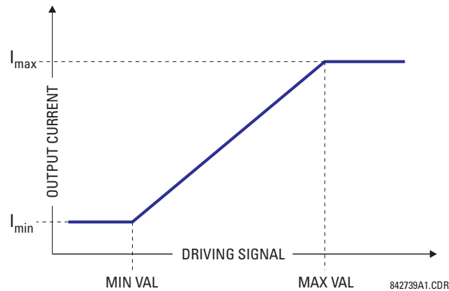
Figure 5-107: DCMA OUTPUT CHARACTERISTIC
