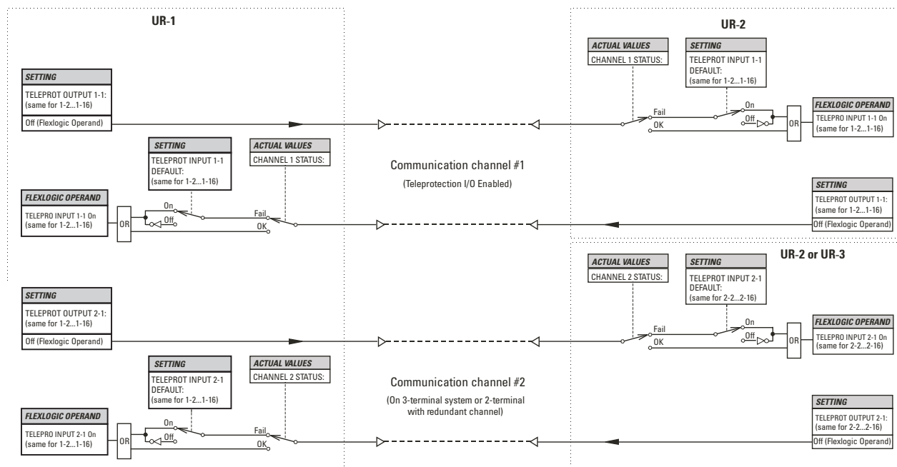
Figure 5-106: TELEPROTECTION INPUT/OUTPUT PROCESSING
