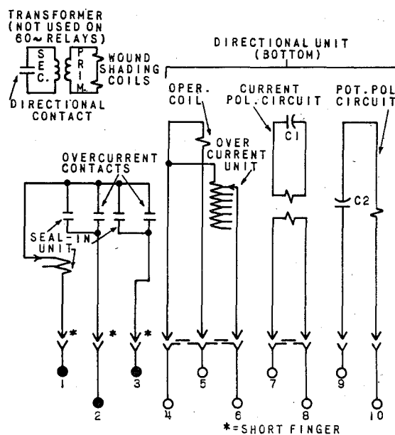
Fig. 17 Internal Connections For The Type IBC652A Relay (Front View)
