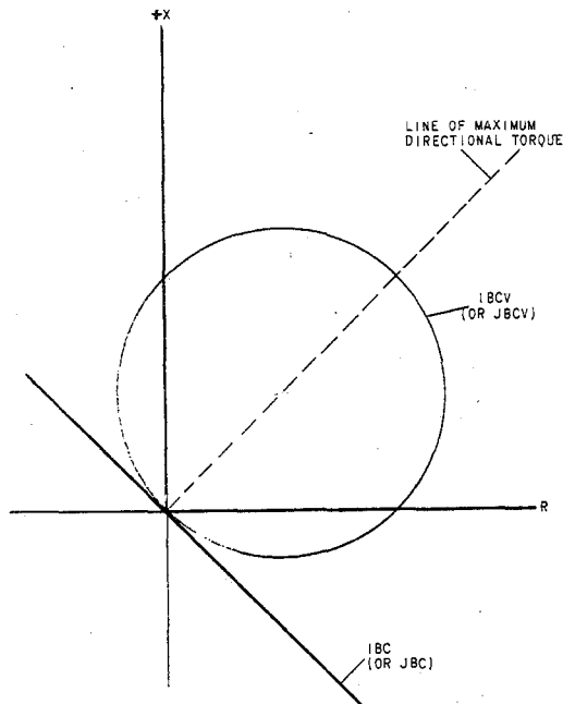
Fig. 2 Impedance Characteristics Of The Type IBC And IBCV Relays
