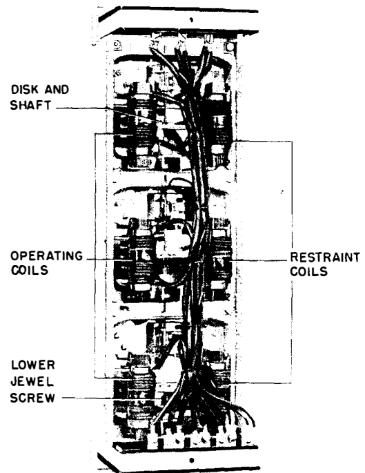
Fig. 5 (8007883) Type IJC51B Relay-Unit in Cradle (Rear View)
